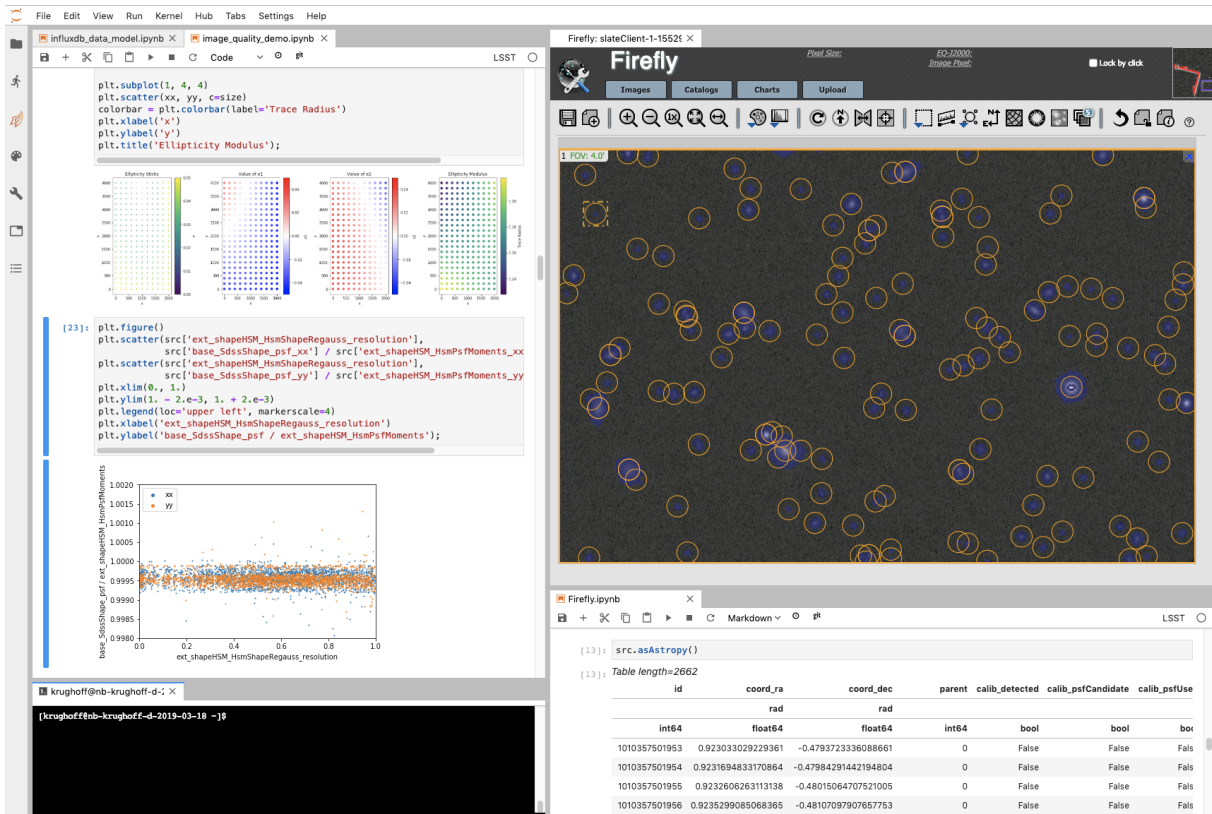
FIGURE 4: A screen capture of the Notebook interface running LSST image processing code within a notebook.
